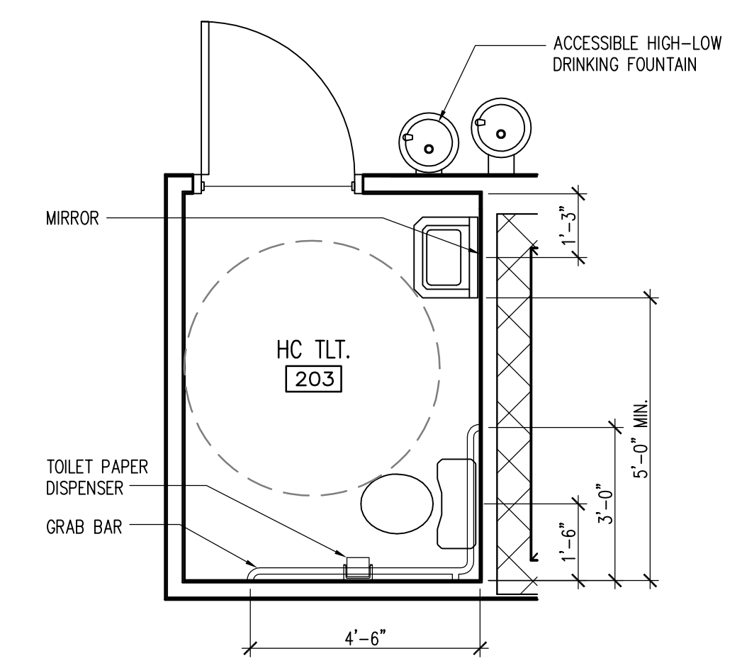
ENLARGED TLT. RM. PLAN
