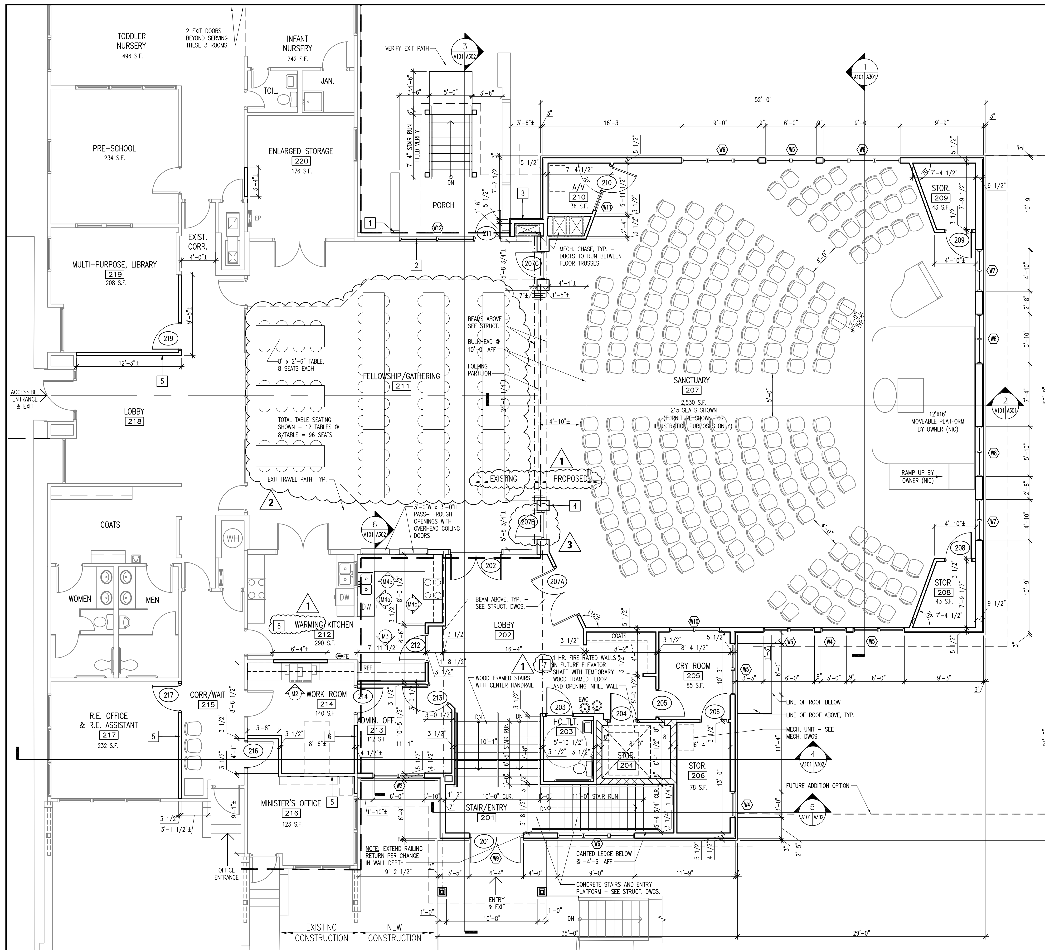
MAIN LEVEL FLOOR PLAN
